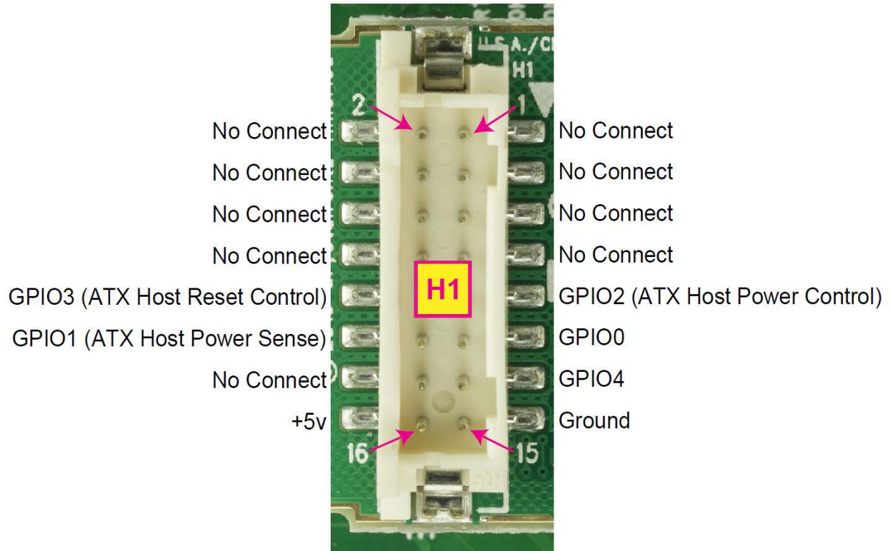
Figure 7. Pin Assignments on CFA635-xxx-KU H1 Connector
