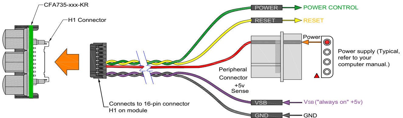
Figure 15. ATX Power Supply and Control Connections Using Crystalfontz WR-PWR-Y25 Cable
