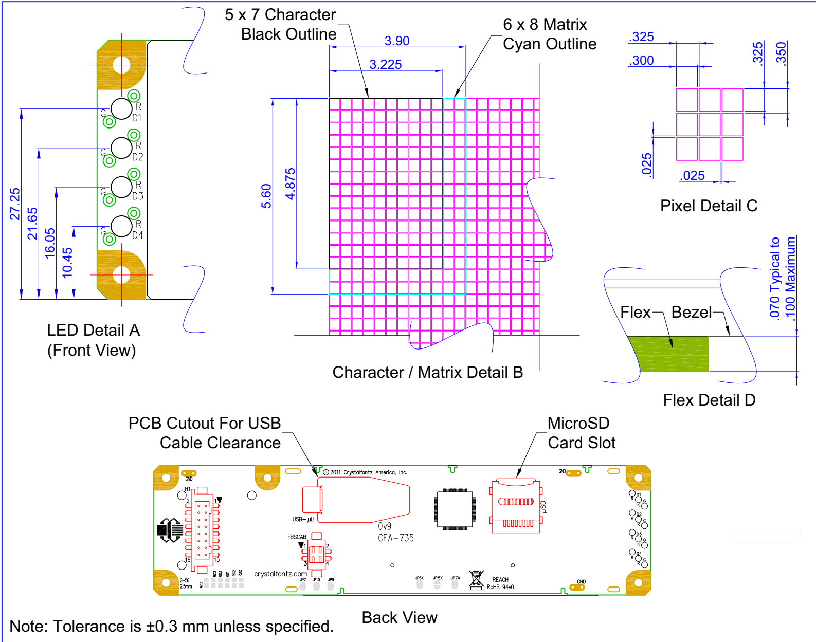
Figure 3. Module Outline Drawing Back View and Pixel Detail
