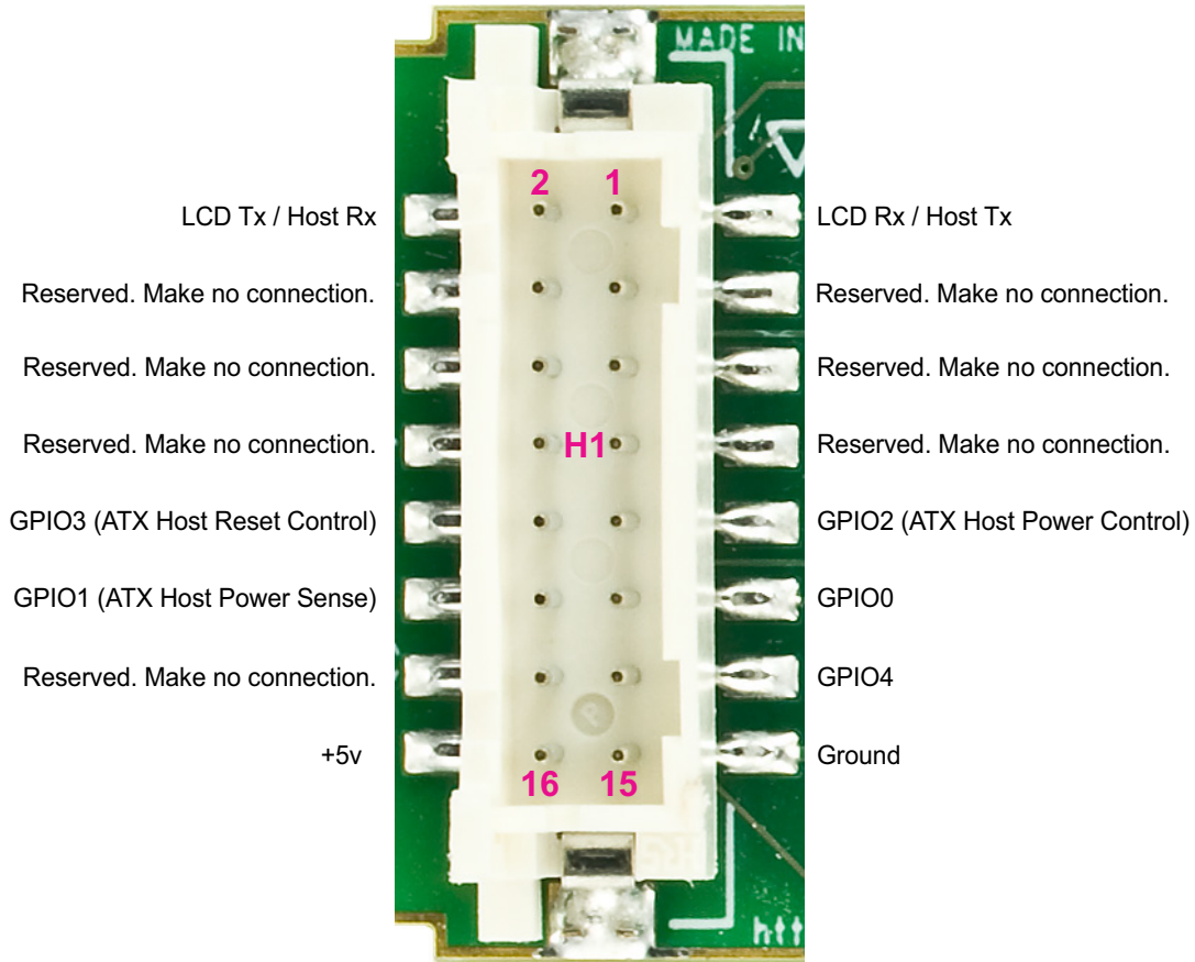
Figure 16. Pin Assignments on CFA735-xxx-KR's H1 Connector (Includes GPIOs)
