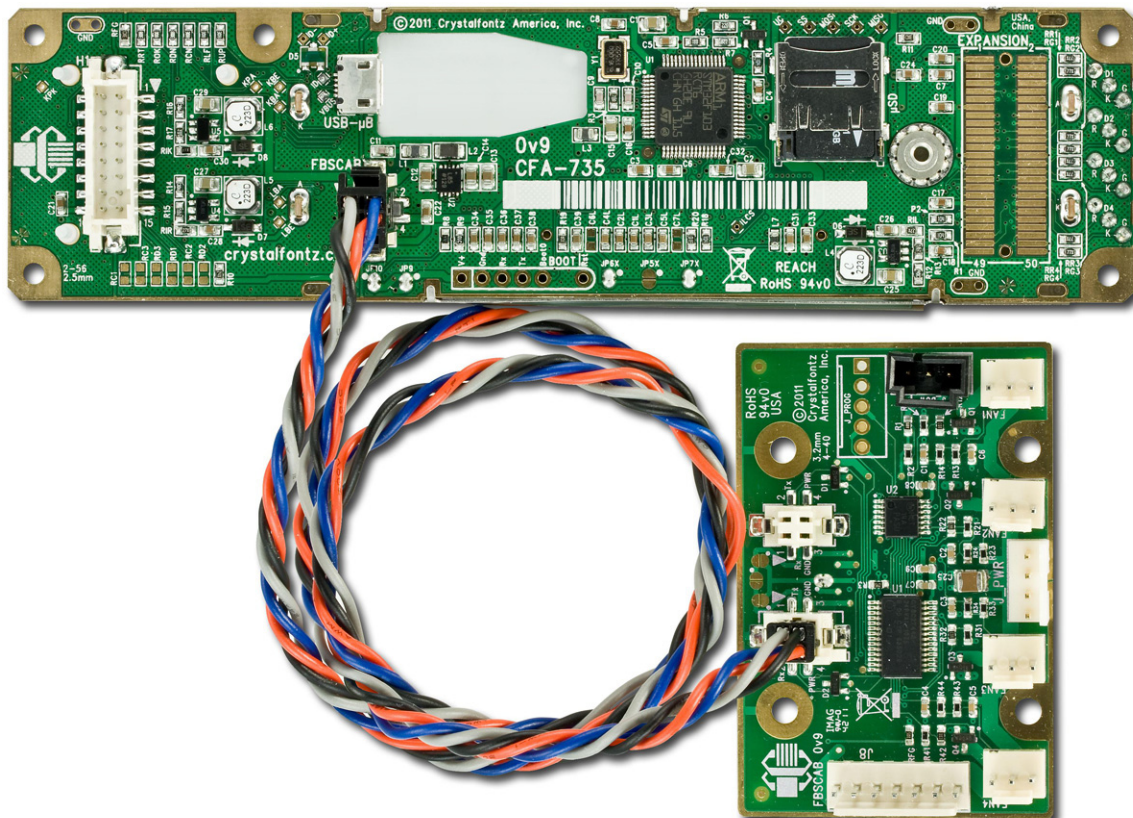
Figure 17. CFA735-xxx-KR Module Connected to Optional CFA-FBSCAB with WR-EXT-Y37 Cable
