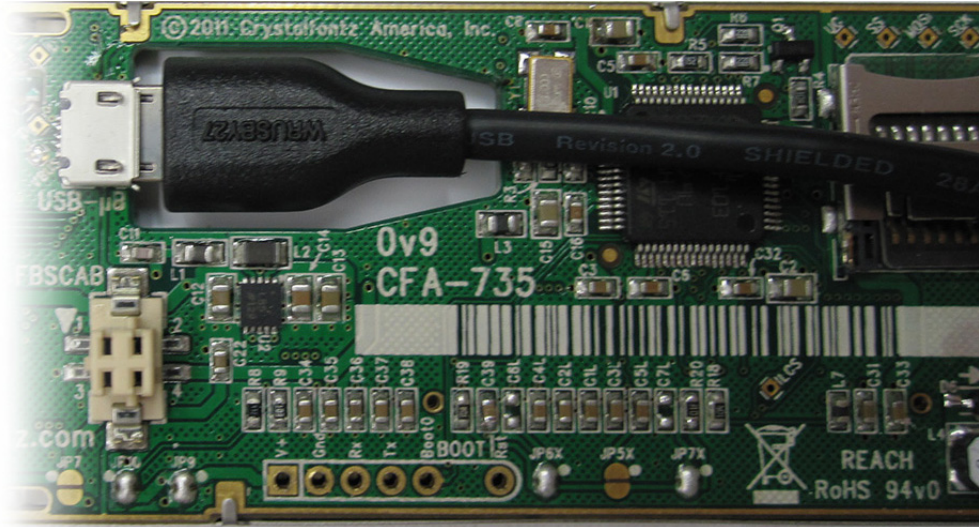
Figure 14. Standard (+5v) Power Supply and USB Data Communications through USB
