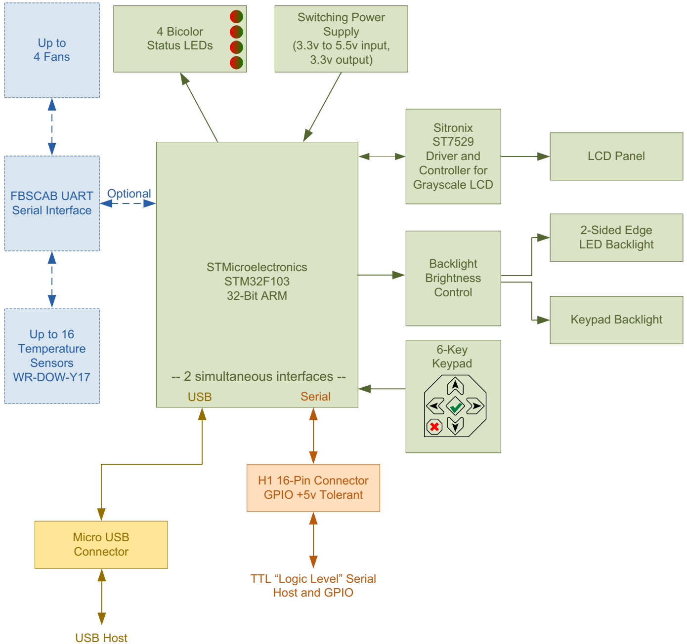
Figure 6. System Block Diagram
