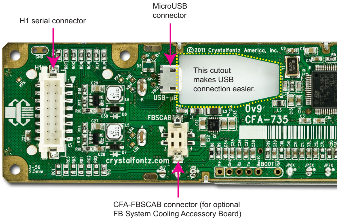
Figure 13. Location of Connectors
