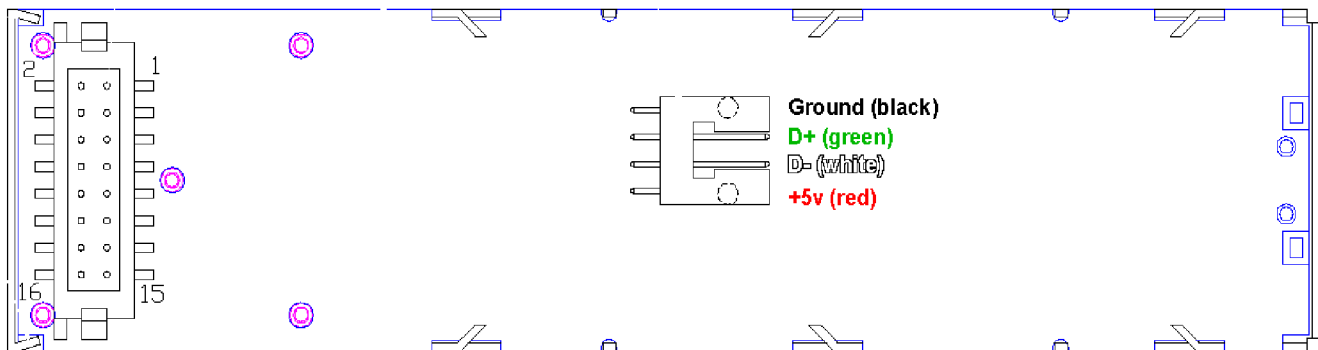
Figure 2. CFA631-RMF-KU USB Host Connection
