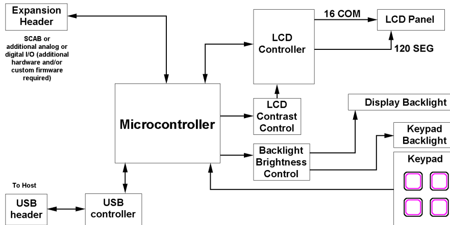
Figure 1. CFA631-RMF-KU System Block Diagram
